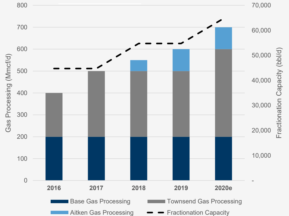
Operational Capacity (Fractionation and NEBC Processing Facilities)
